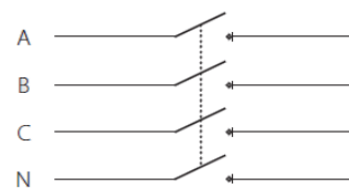
交流四层产品接线图 Cabling across four layers
