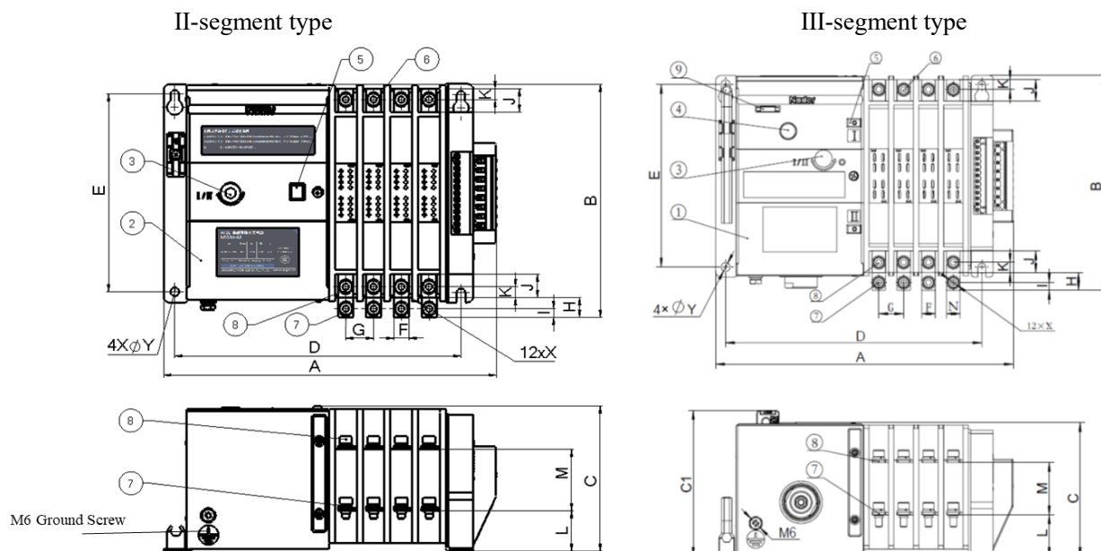
Fig. 2 External dimensions and mounting dimensions of the split switching mechanism body
