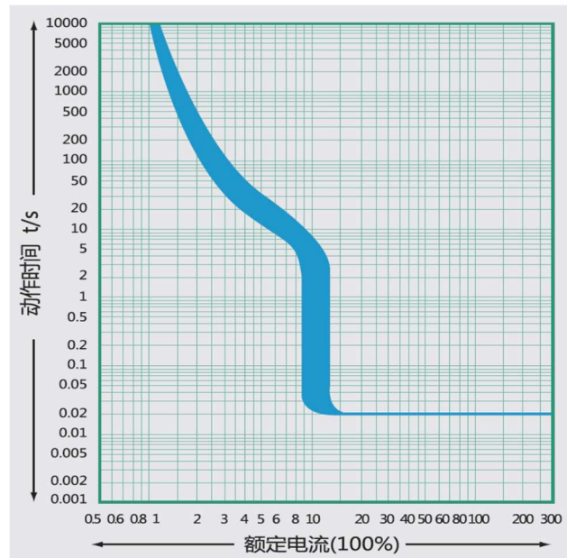
时间/电流特性曲线 Time/Current Characteristic Curve
