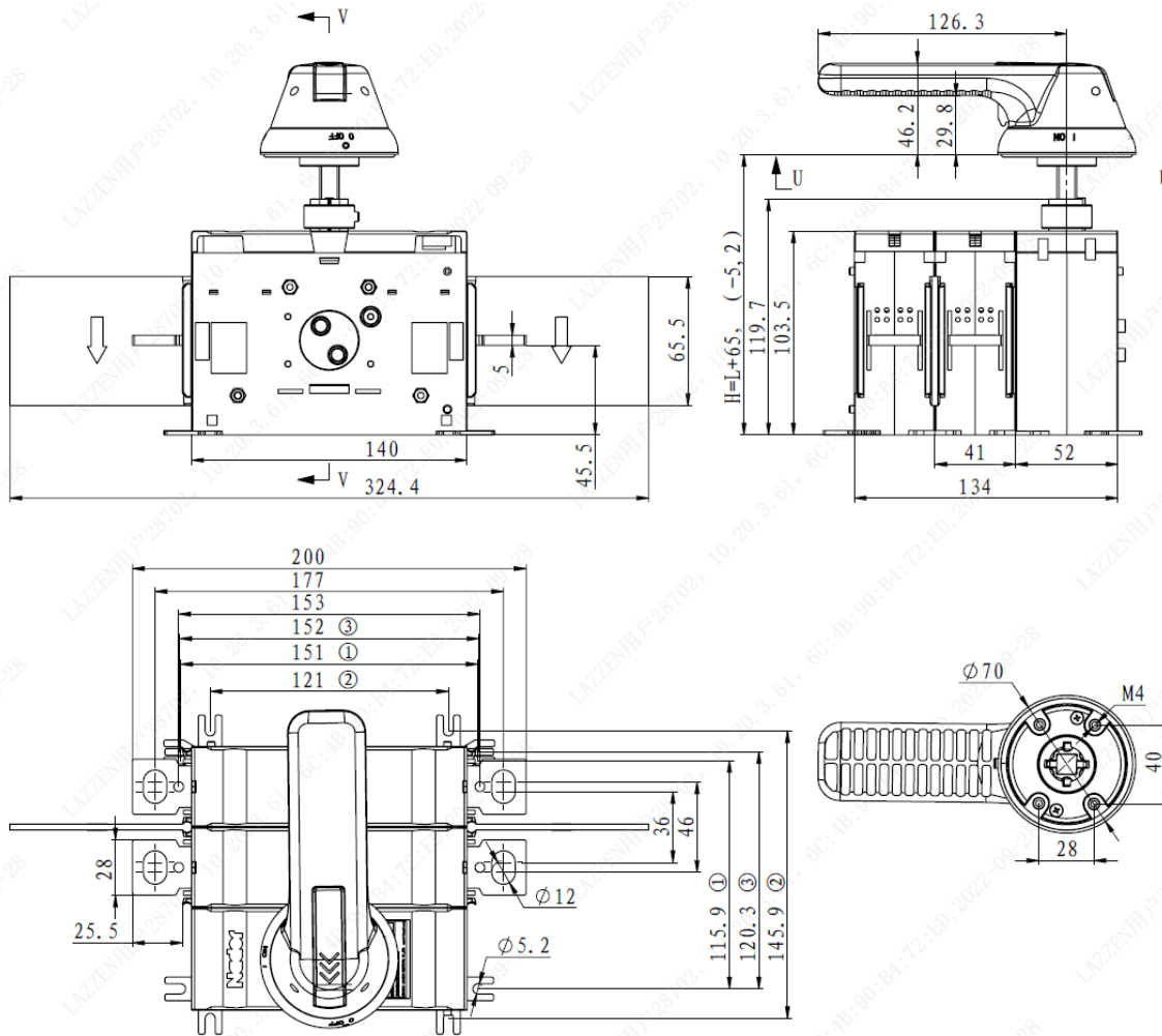
Standard operation outline installation drawing
