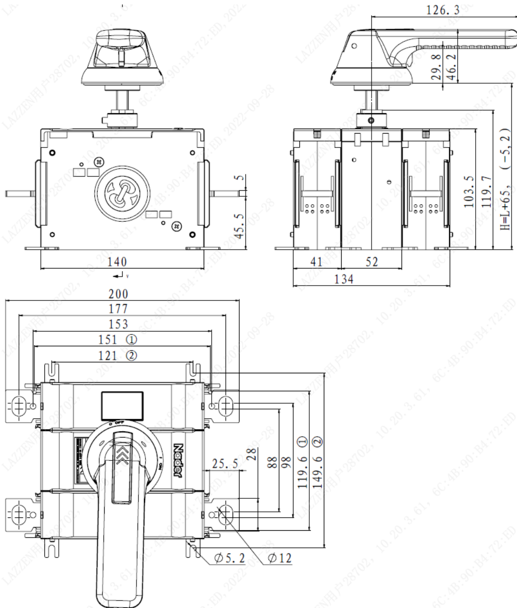
Standard Operation (Mechanism Centered) Outline Installation Drawing
