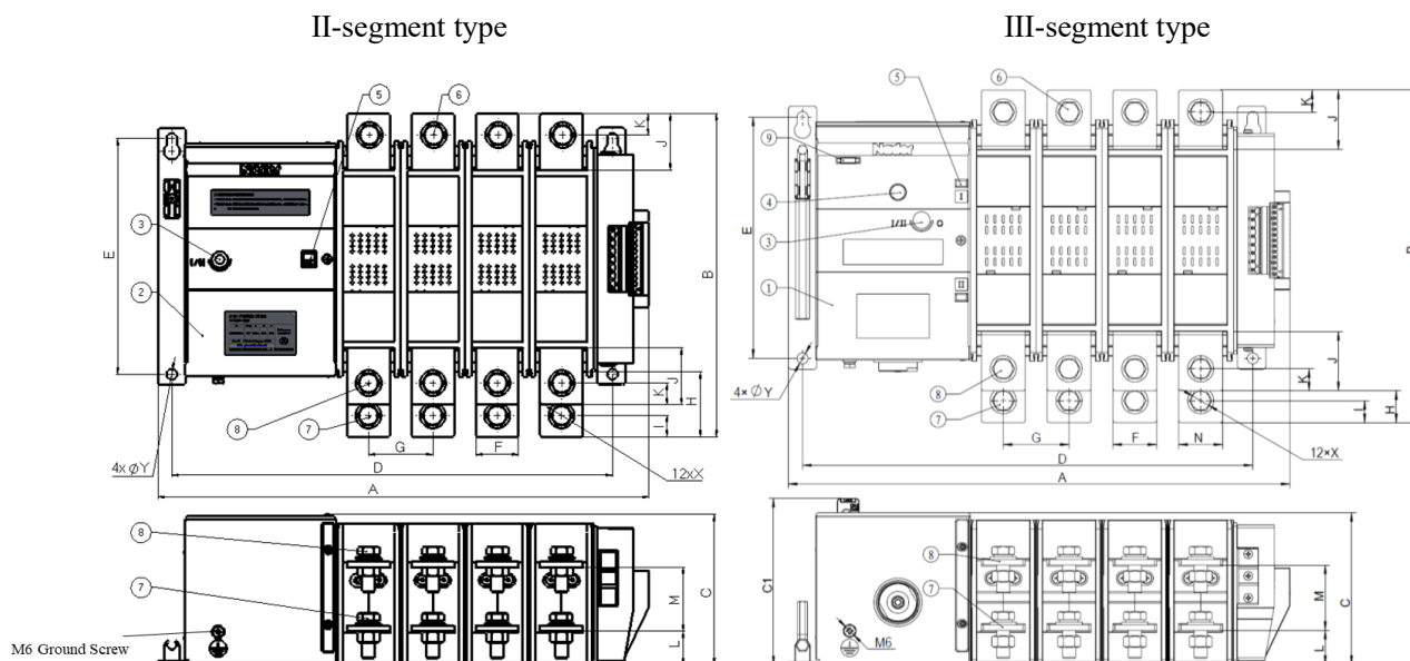
Fig. 2 External dimensions and mounting dimensions of the split switching mechanism body
