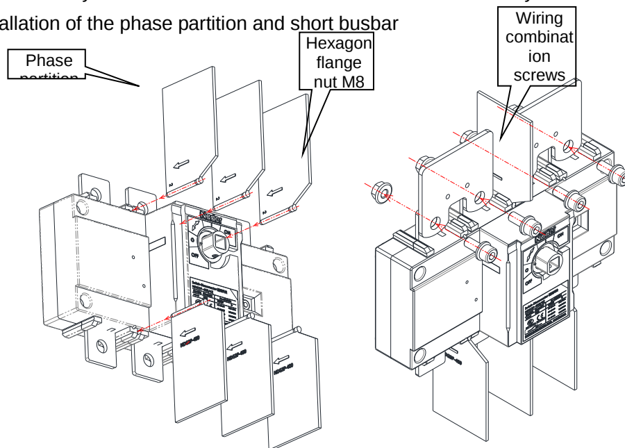
Installation of the phase partition for the basic product
