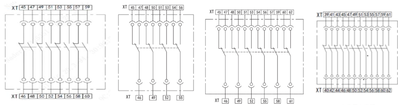
Four normally opened and four normally closed NDW2G-4000
