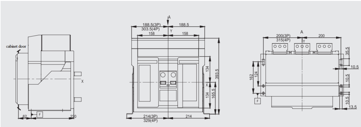
800A-2500A Horizontal Wiring, Vertical Wiring
