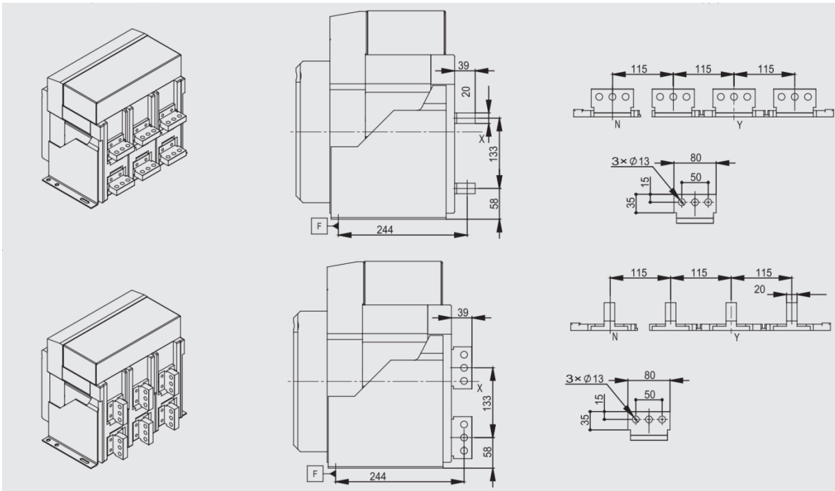
800A-2500A Horizontal Wiring, Vertical Wiring
