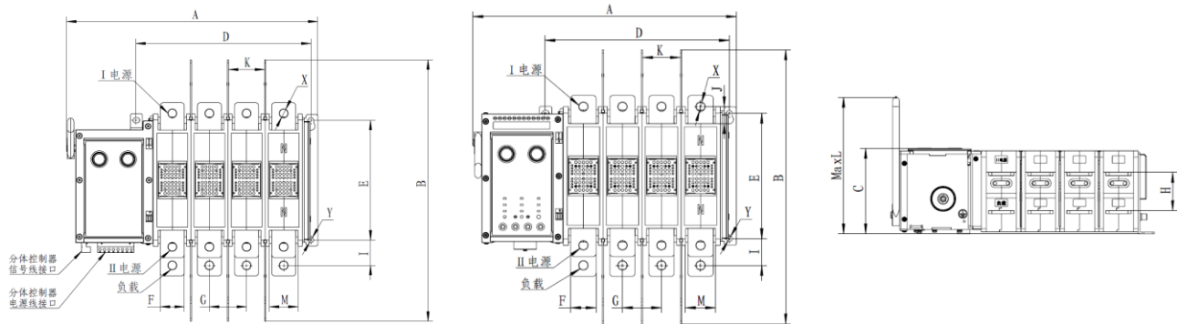
Split appearance diagram (including D-type split body) Overall appearance diagram
