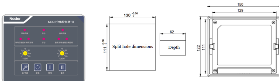
Fig.13 Shape and size of the N-type/blank split controller
