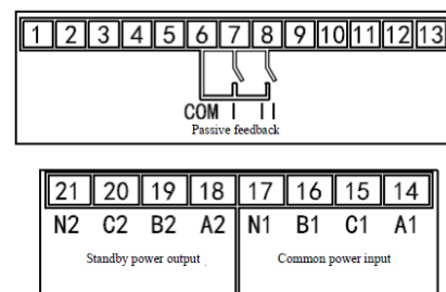
Fig.8 Schematic diagram of secondary terminal of blank II-segment split controller
