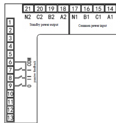
Fig.10 Schematic diagram of the secondary terminal of N-type III-segment split controller
