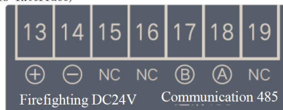
Fig.6 N-type overall communication auxiliary terminal diagram
