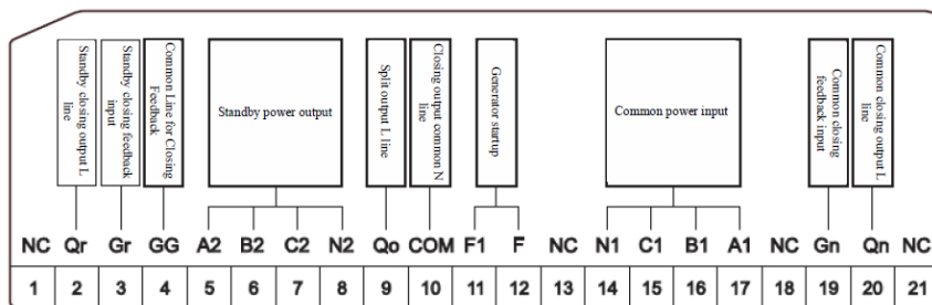
Fig.8 Schematic diagram of secondary terminal of blank II-segment split controller
