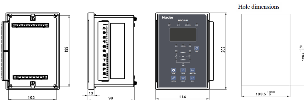
Fig.14 Installation dimensions of D-type controller
