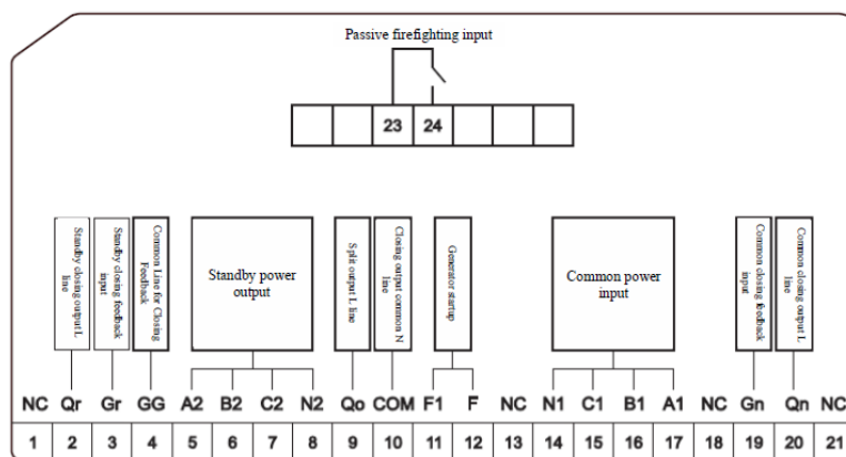
Fig.10 Schematic diagram of the secondary terminal of N-type III-segment split controller
