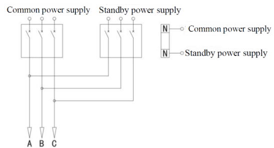
Fig.2 Schematic diagram of three-pole product wiring
