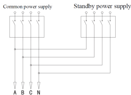
Fig.1 Schematic diagram of four-pole product wiring
