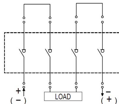
Lower wiring of 4P in series
