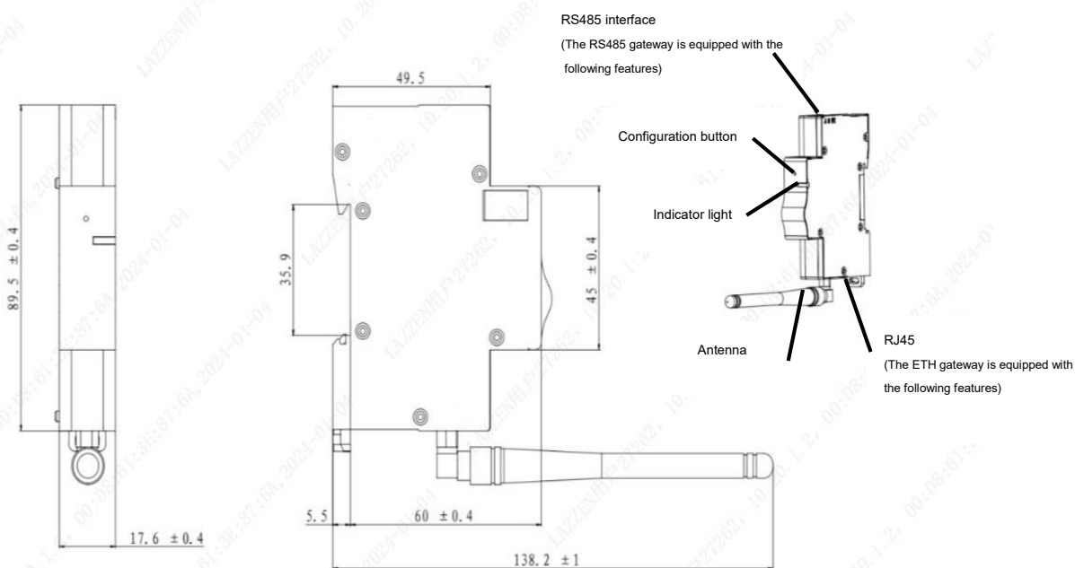
Outline and Installation Dimension Drawing of DF-TMB Gateway Module
