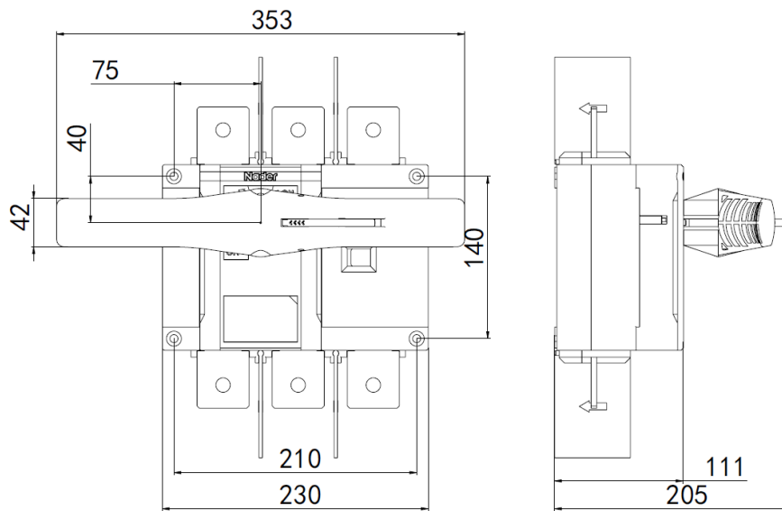
6.4 Cabinet door opening dimension diagram of handle outside a cabinet: SB1-"A"/G3-800
