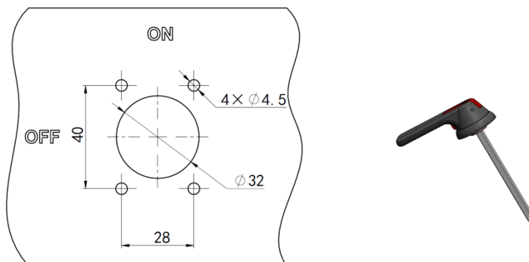
6.5 Cabinet door opening dimension diagram of handle outside a cabinet: SB1-"A"/G3A-800
