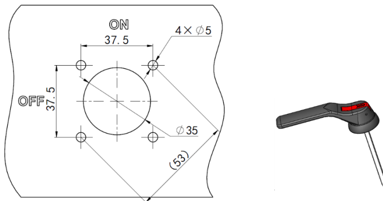
6.5 Cabinet door opening dimension diagram of handle outside a cabinet: SB1-"A"/G3A-800
