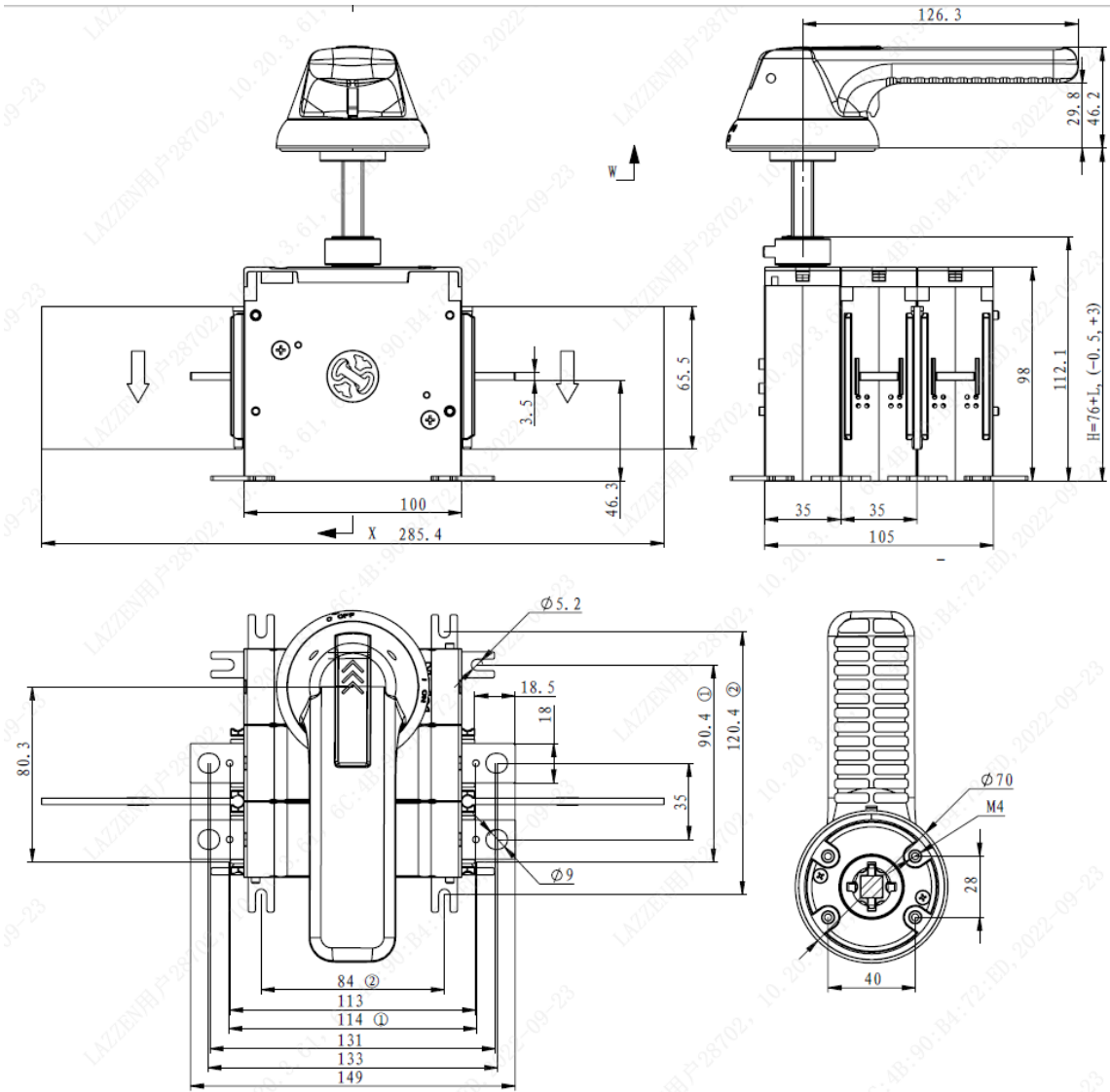
Standard operation outline installation drawing
