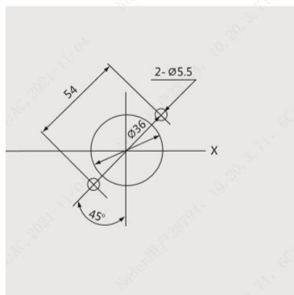
CS1-A handle switchgear door recommended opening diagram, 2×M4 mounting screw torque 1.5-1.6N.m,
