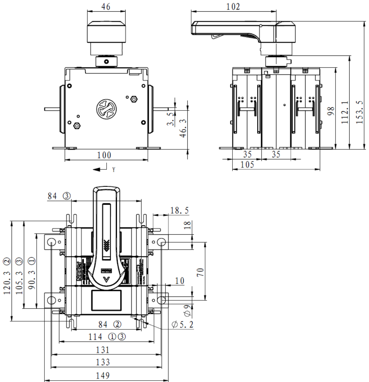
Forward operation (center of cabinet mechanism) Outline installation drawing (opening)
