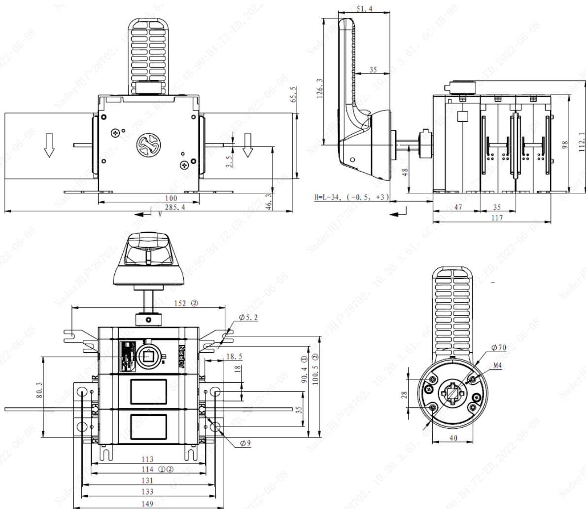
Side operation outline installation drawing
