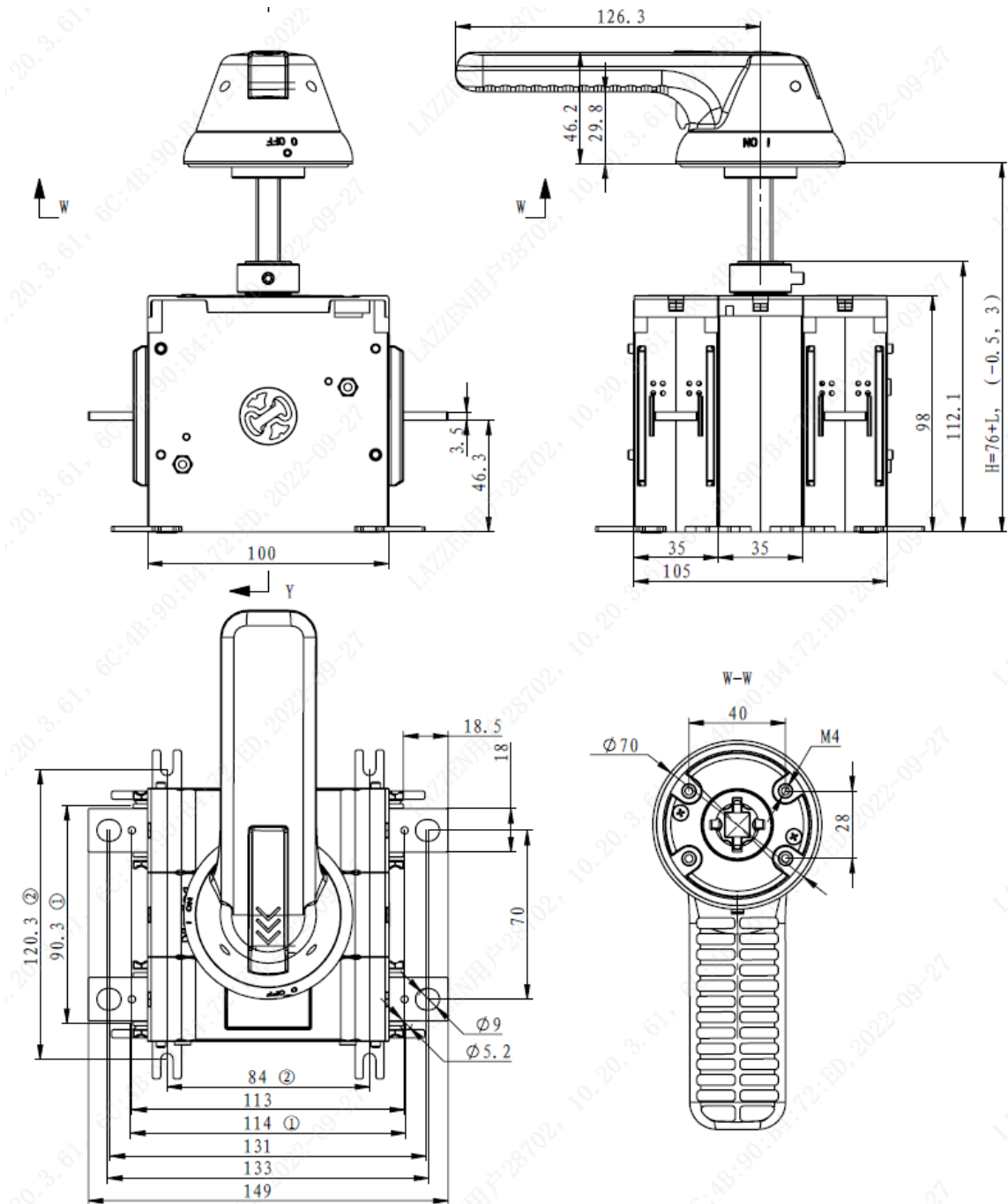
Standard Operation (Mechanism Centered) Outline Installation Drawing
