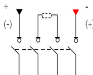
Four-pole string connection mode
