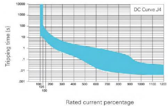
J4 Curve
