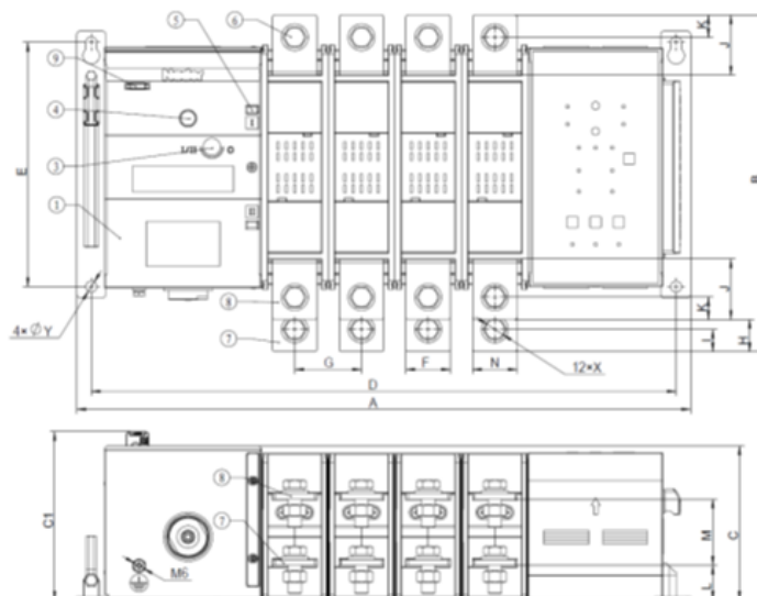
Fig. 1 External Dimensions and Installation Dimensions of the Integral Switch
