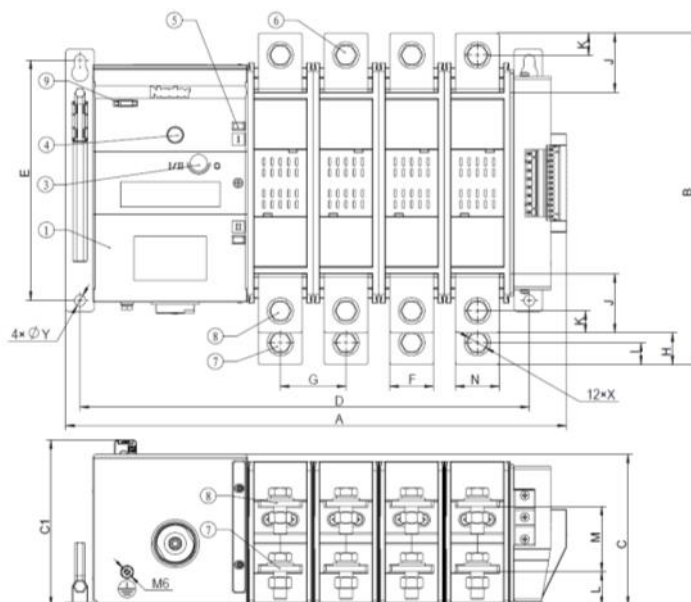
Fig. 2 External dimensions and mounting dimensions of the split switching mechanism body
