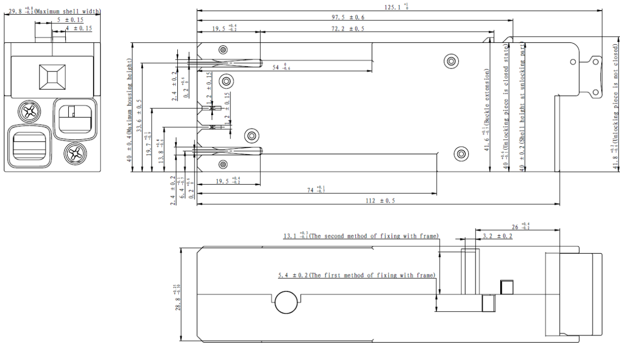
NDB6AZ-125H Outline and installation dimensions
