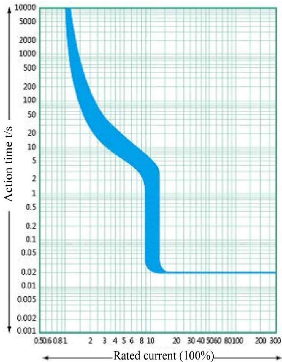
Time/Current Characteristic Curve
