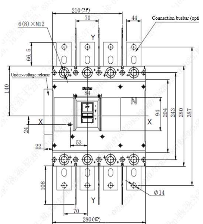
2P+N/3P/4P
