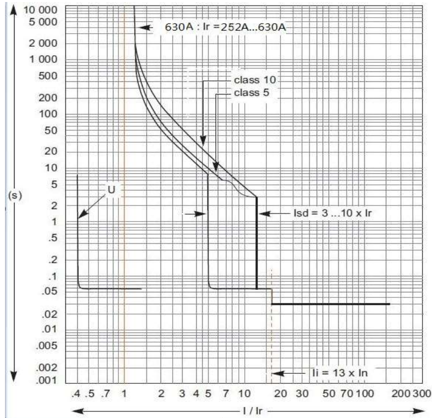
Motor protection type Characteristic Curve
