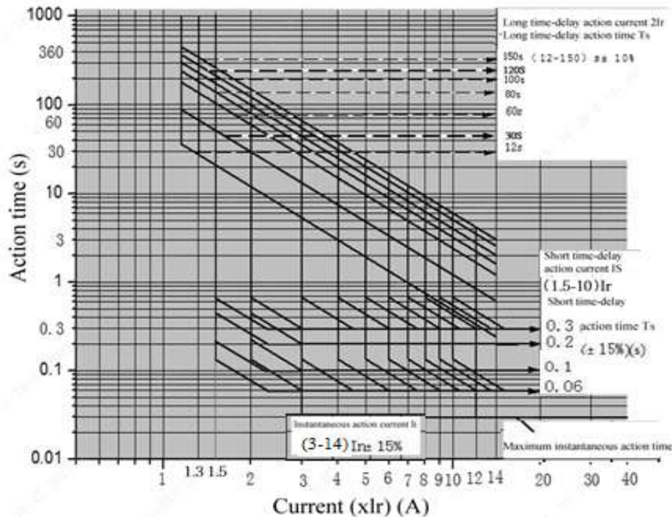
Time/Current Characteristic Curve
