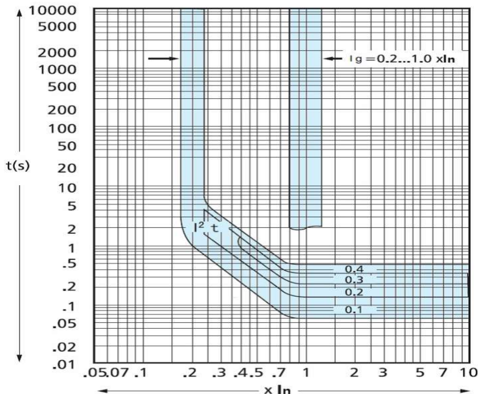
Ground protection characteristic curve
