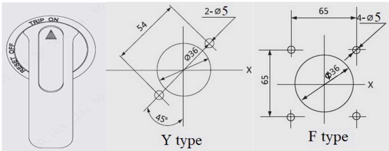
Fig 26 Installation holes of rotary handle
