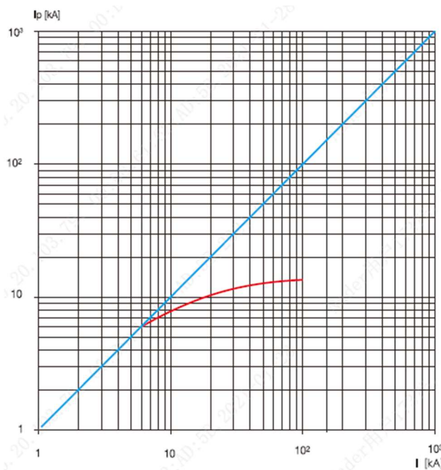
Fig 6 NDM5Z-400 current-limiting curves (DC1000V 4 poles in series)
