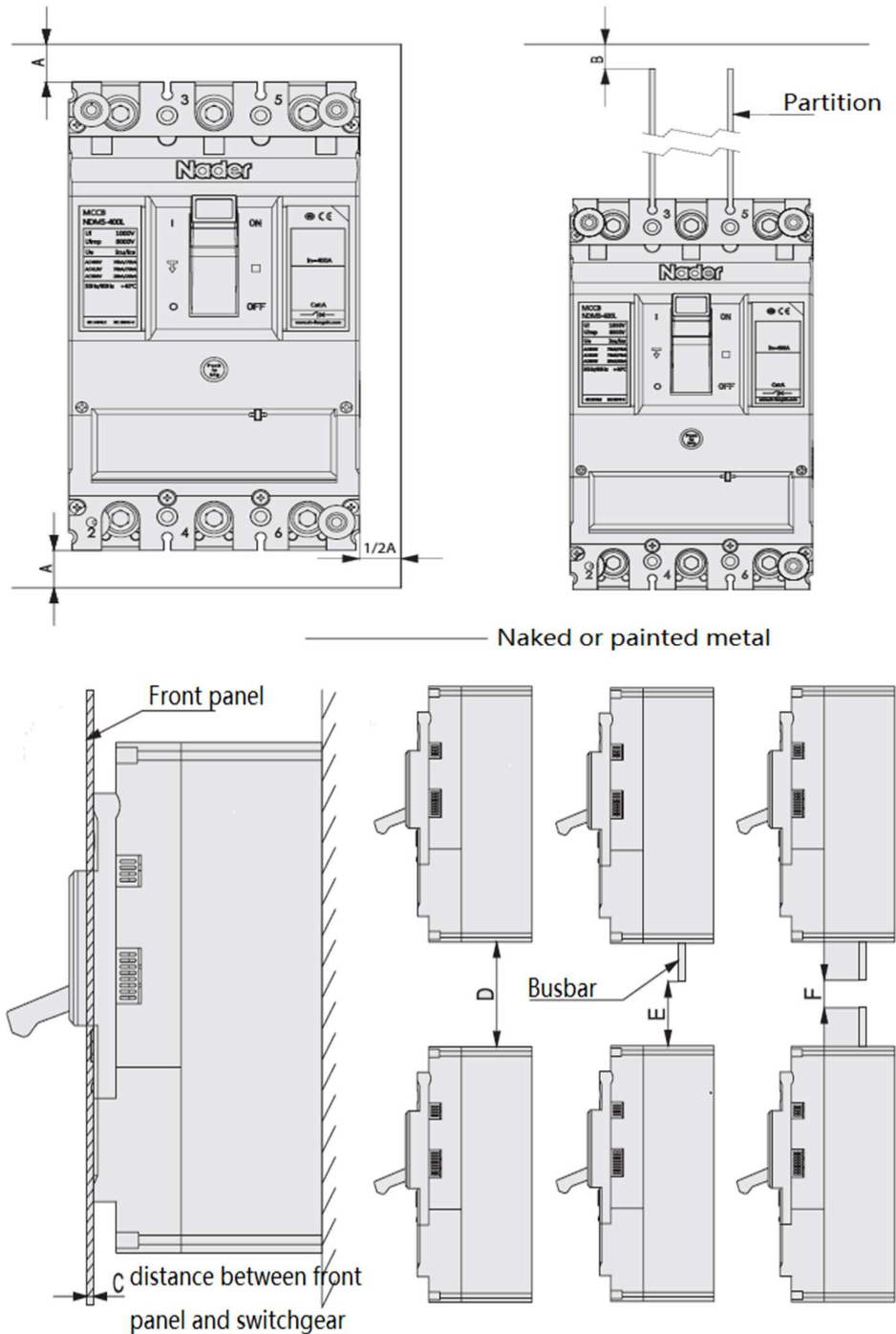
Figure 30 diagram when circuit breaker installation;
