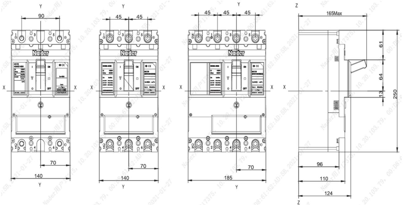
Fig 13 NDM5Z-630 outline dimensions of 2-pole, 3-pole and 4-pole front panel connection products
