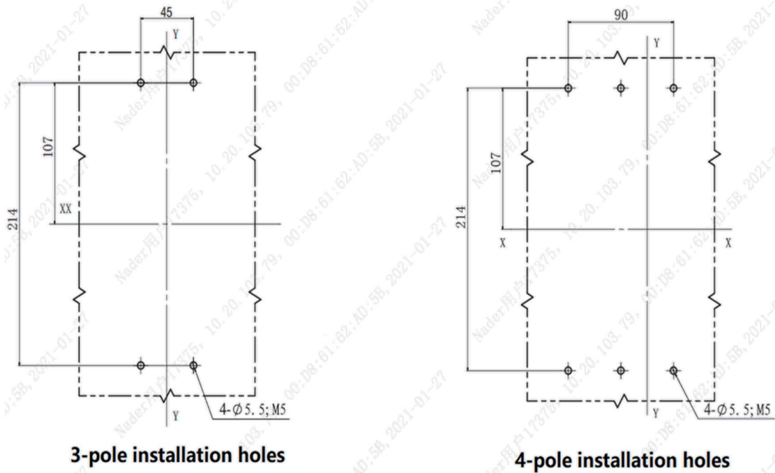
Fig 12 NDM5Z installation dimensions of 3-pole and 4-pole front panel connection products
