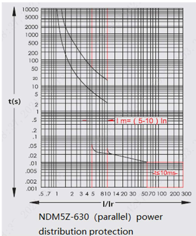
Fig 5 tripping curves
