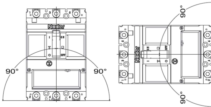
Fig 34 diagram of installation direction Vertical installation (upright) Horizontal installation (level)
