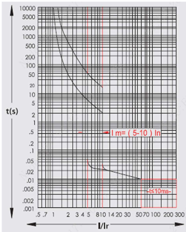
Fig 3 tripping curves of NDM5Z-400
