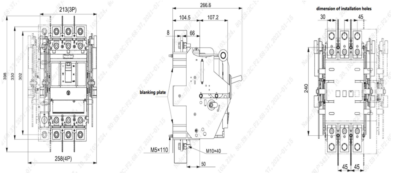
Fig 22 Outline and installation dimensions of 3-pole and 4-pole front panel connection products with drawer
