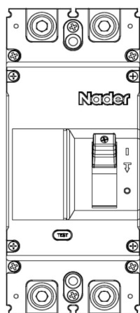
Vertical Installation
