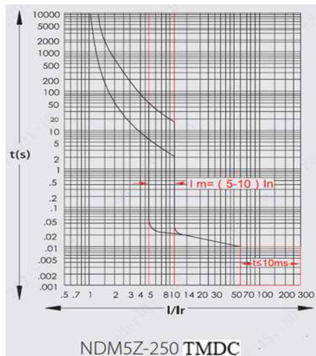
Fig.3 Trip curve
