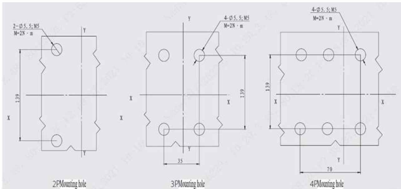
Fig. 9 2P 3P 4P Installation dimension drawing of front board wiring products
