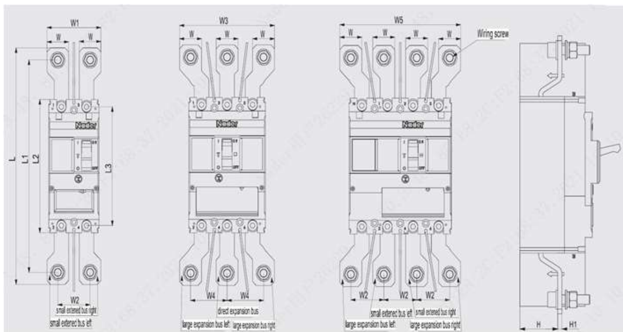
Fig. 10 2P、3P、4P Outline and installation dimensions of expansion wiring in front of the board
