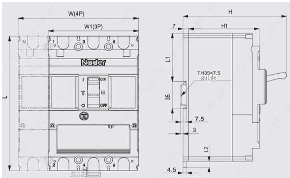
Fig.16 Outline and installation dimensions drawing of guide rail type safety rotation products
