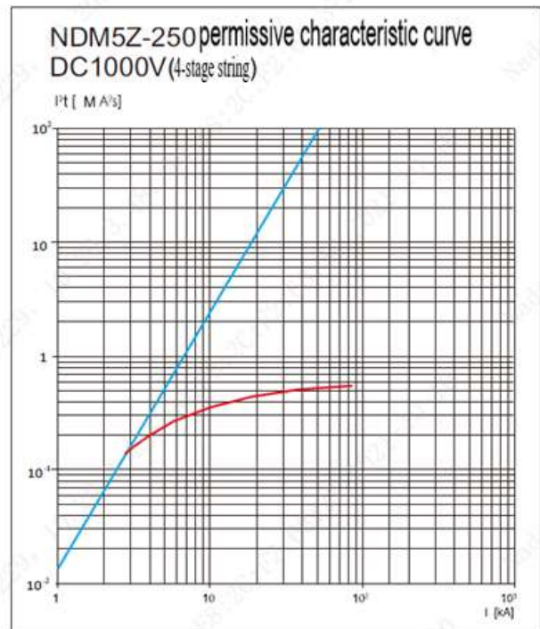
Fig.5 Permissive characteristic curve chart
