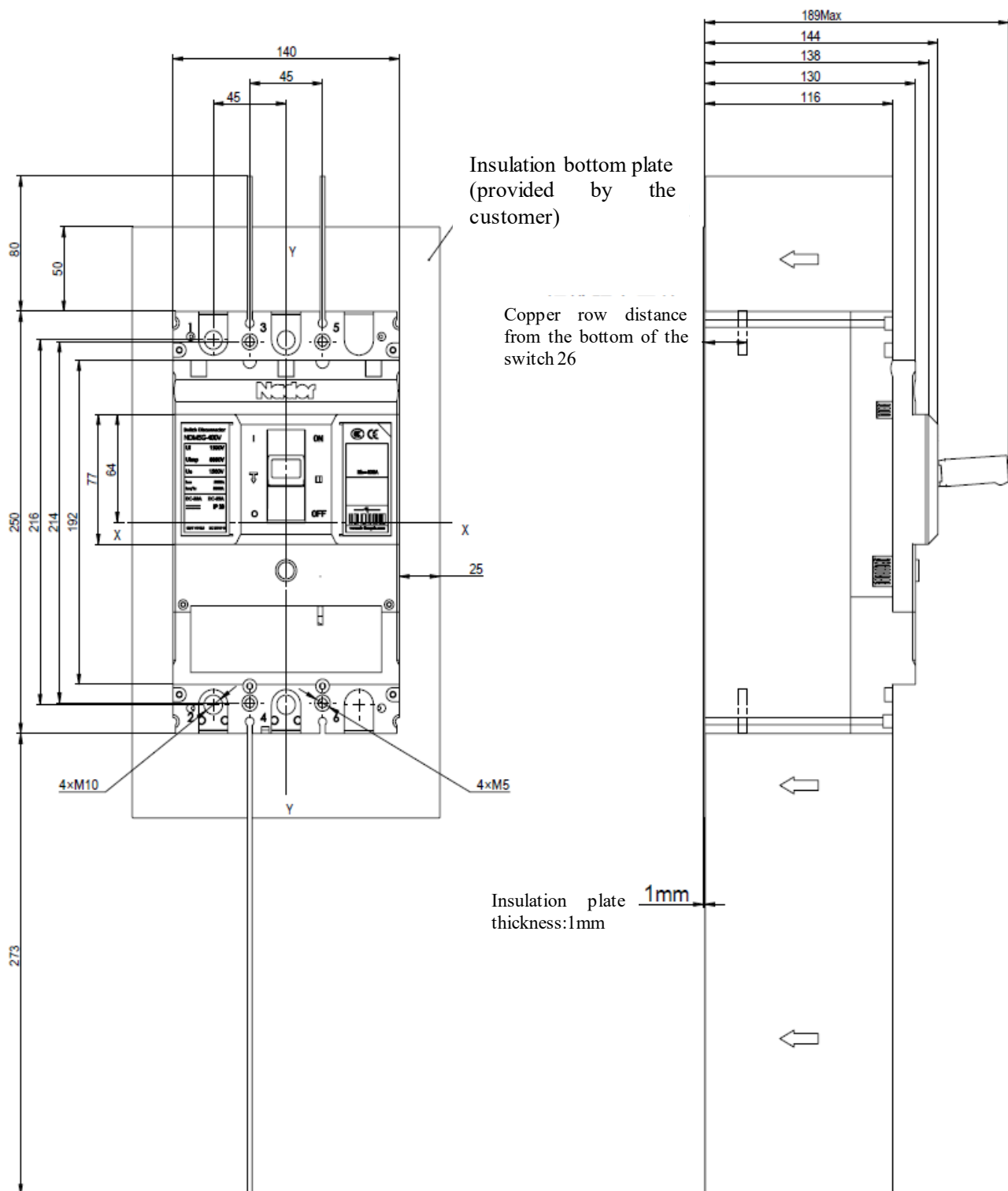
Figure 2 outline dimensions of front-plate connection product
