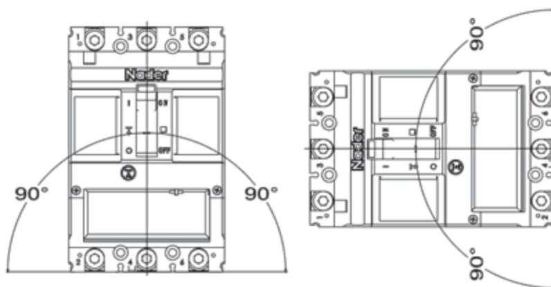
Vertical installation (upright)
