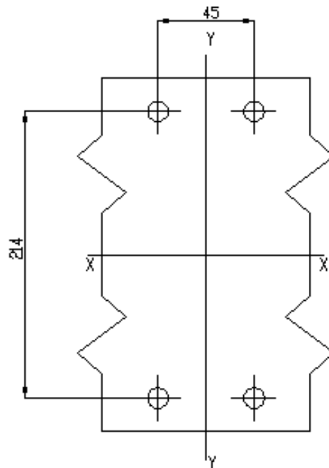
Figure 3 mounting holes dimensions
