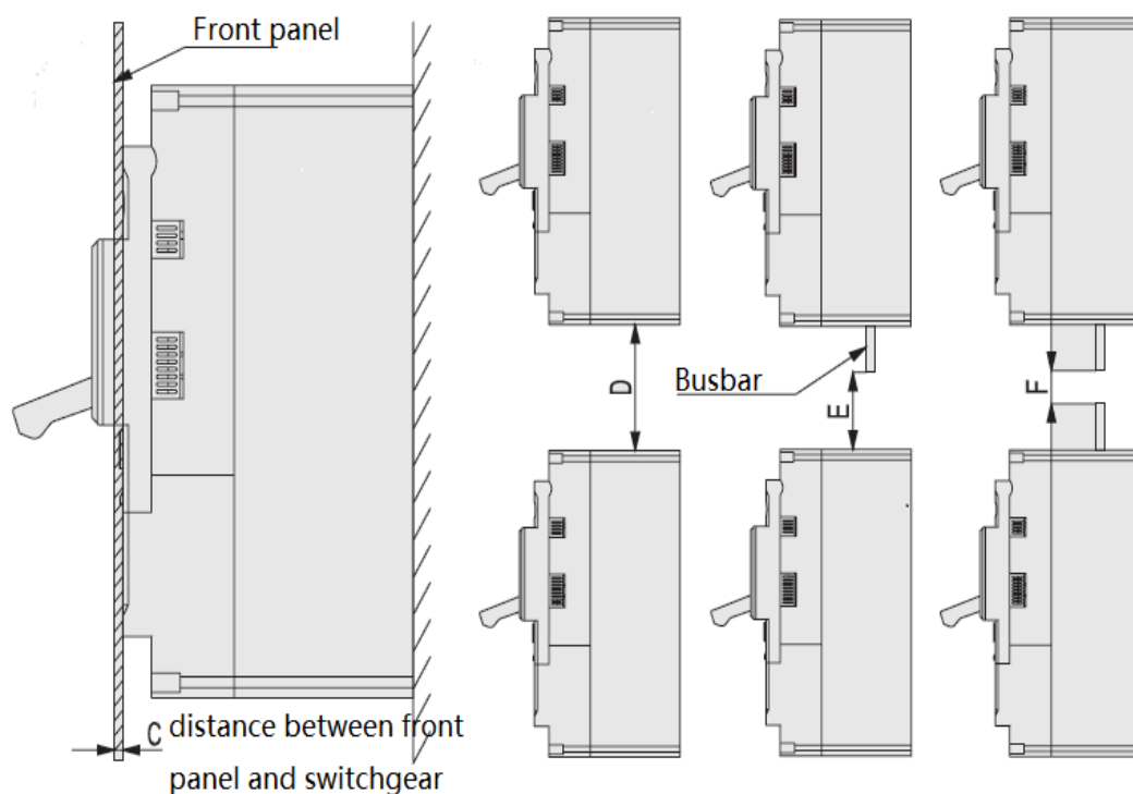
Figure 4 safety spacing
