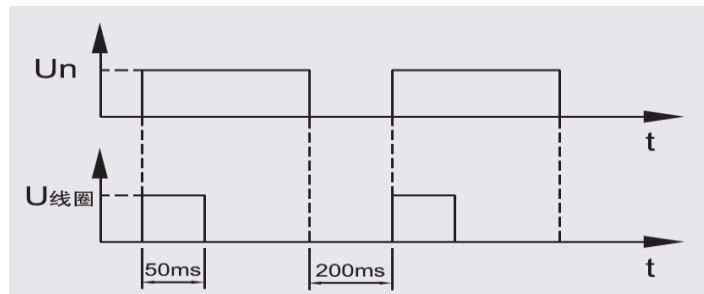
Figure 6 working principle diagram of shunt release
