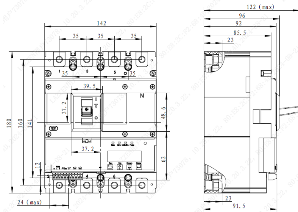
250-4P External Dimensions
