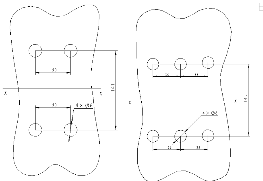
250-3P Mounting Dimensions 250-4P Mounting Dimensions
