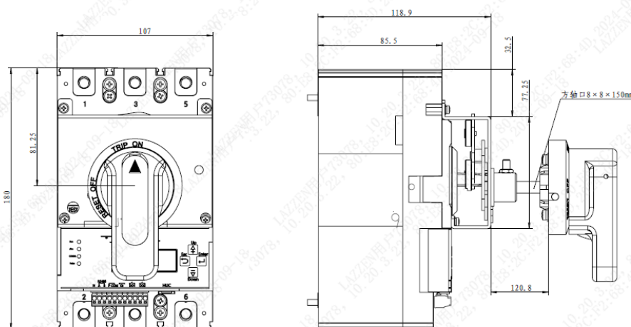
250 External Dimension Diagram of Manual Operation
