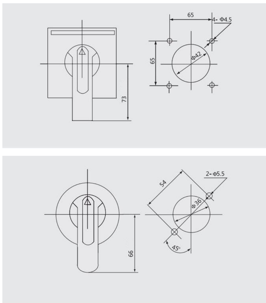
250 Handle Mounting Hole Diagram
