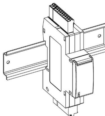
Installation diagram
