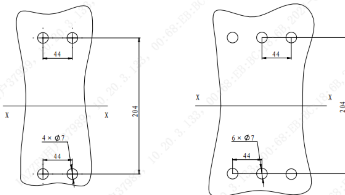
630-3P Mounting Dimensions 630-4P Mounting Dimensions
