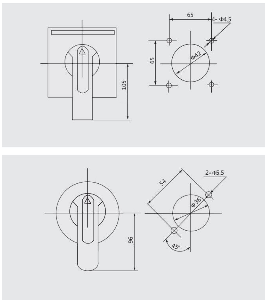
630 Handle Mounting Hole Diagram
