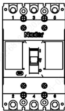
Vertical Installation
