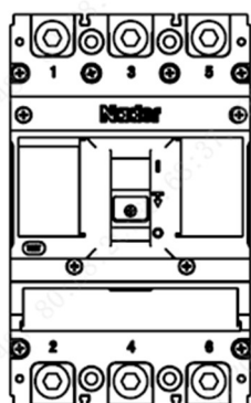
Vertical Installation
