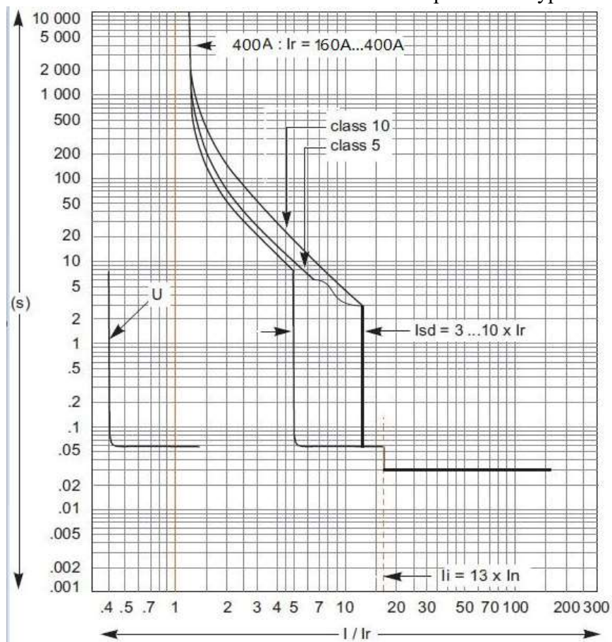
Time/Current Characteristic Curve
