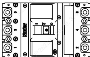
Horizontal Installation
