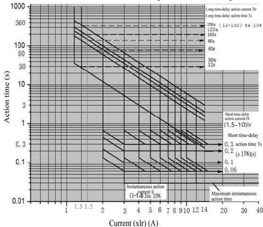
Time/Current Characteristic Curve
