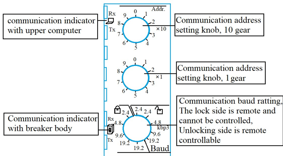
Gear Adjustment of Communication Adaptor
