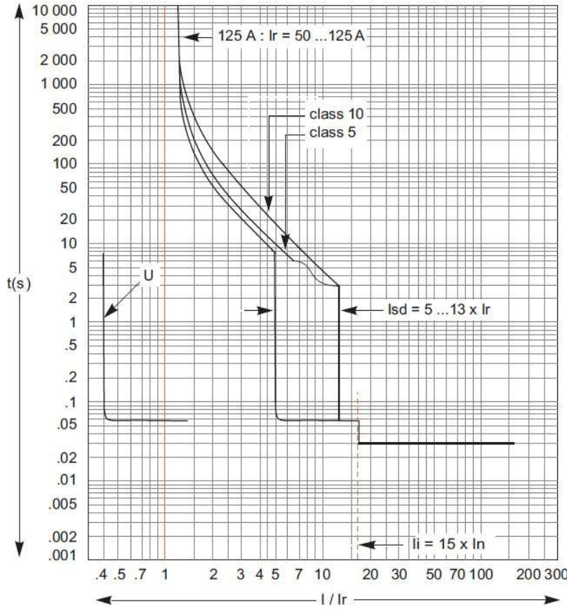
Motor protection Characteristic Curve
