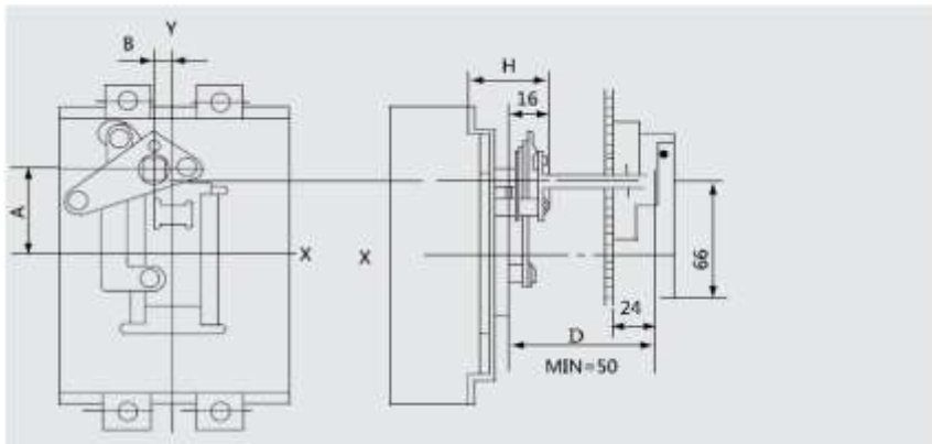
7.2.4 Electric operating mechanism and CS2-F handle
