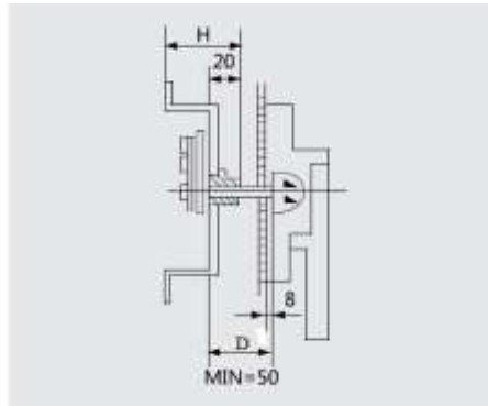
7.2.3 Electric operating mechanism and CS2-A handle
