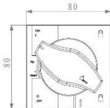
7.2.6 Electric operating mechanism and CS2-IP65 handle
