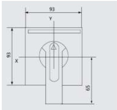
7.2.3 Electric operating mechanism and CS2-A handle
