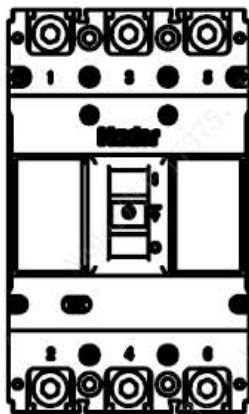
Vertical Installation
