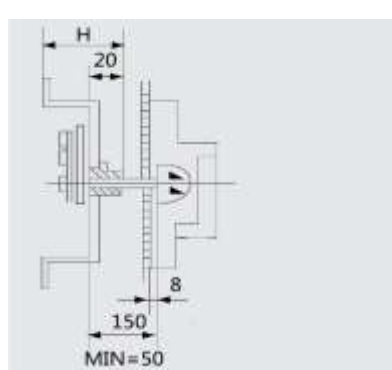
7.2.6 Electric operating mechanism and CS2-IP65 handle
