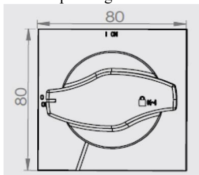
7.6.6 Manual operating mechanism and CS2-IP65 handle
