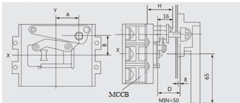
7.5.4 Manual operating mechanism and CS1-IP65 handle
