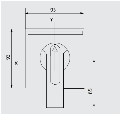
7.5.3 Manual operating mechanism and CS2-A handle
