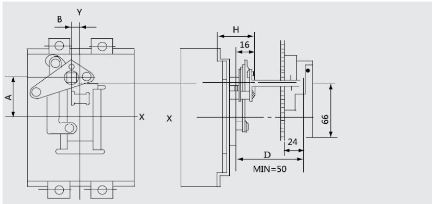
7.5.4 Manual operating mechanism and CS2-F handle
